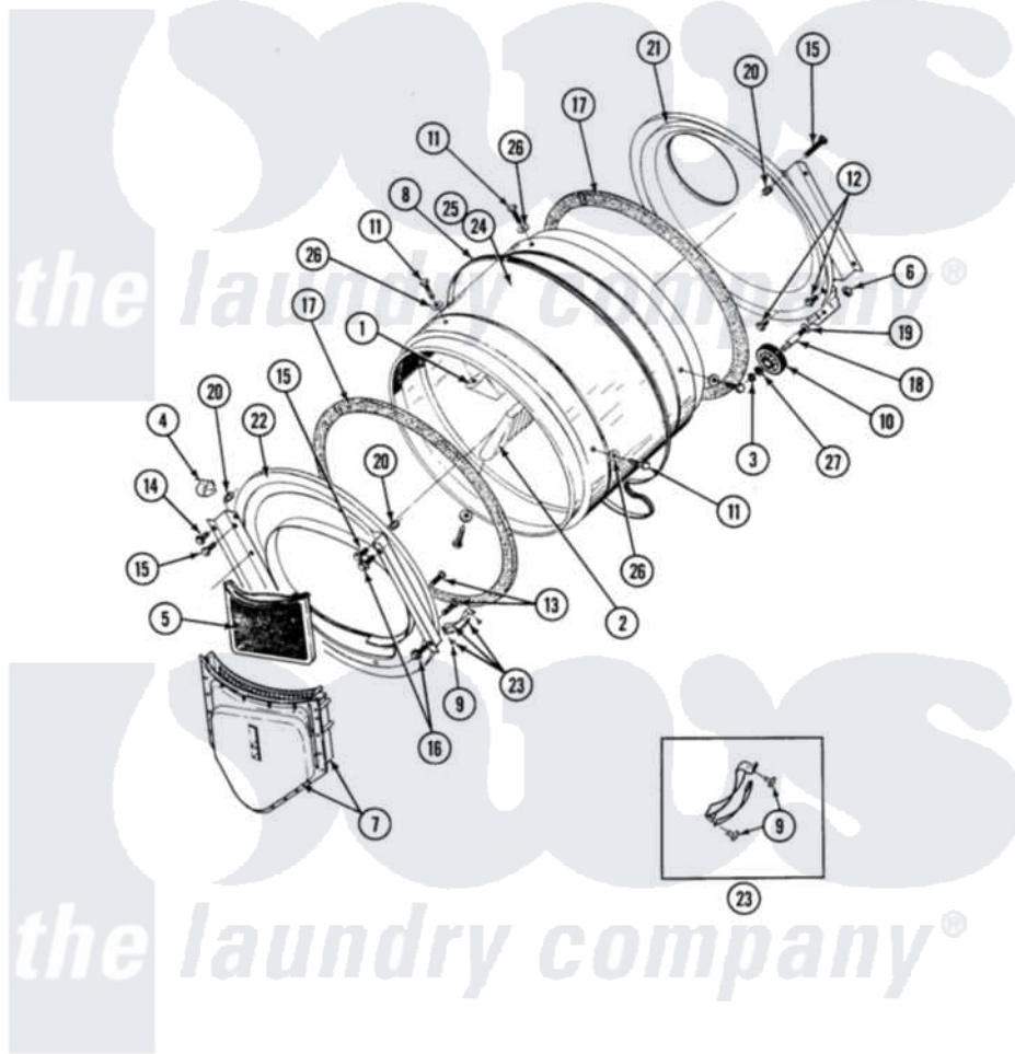
Maytag Commercial Maytag GDG26CS Dryer Parts Parts Diagram 07 - LINT SCREEN, TUMBLER (FRONT & BACK) Click on the part number to view part
