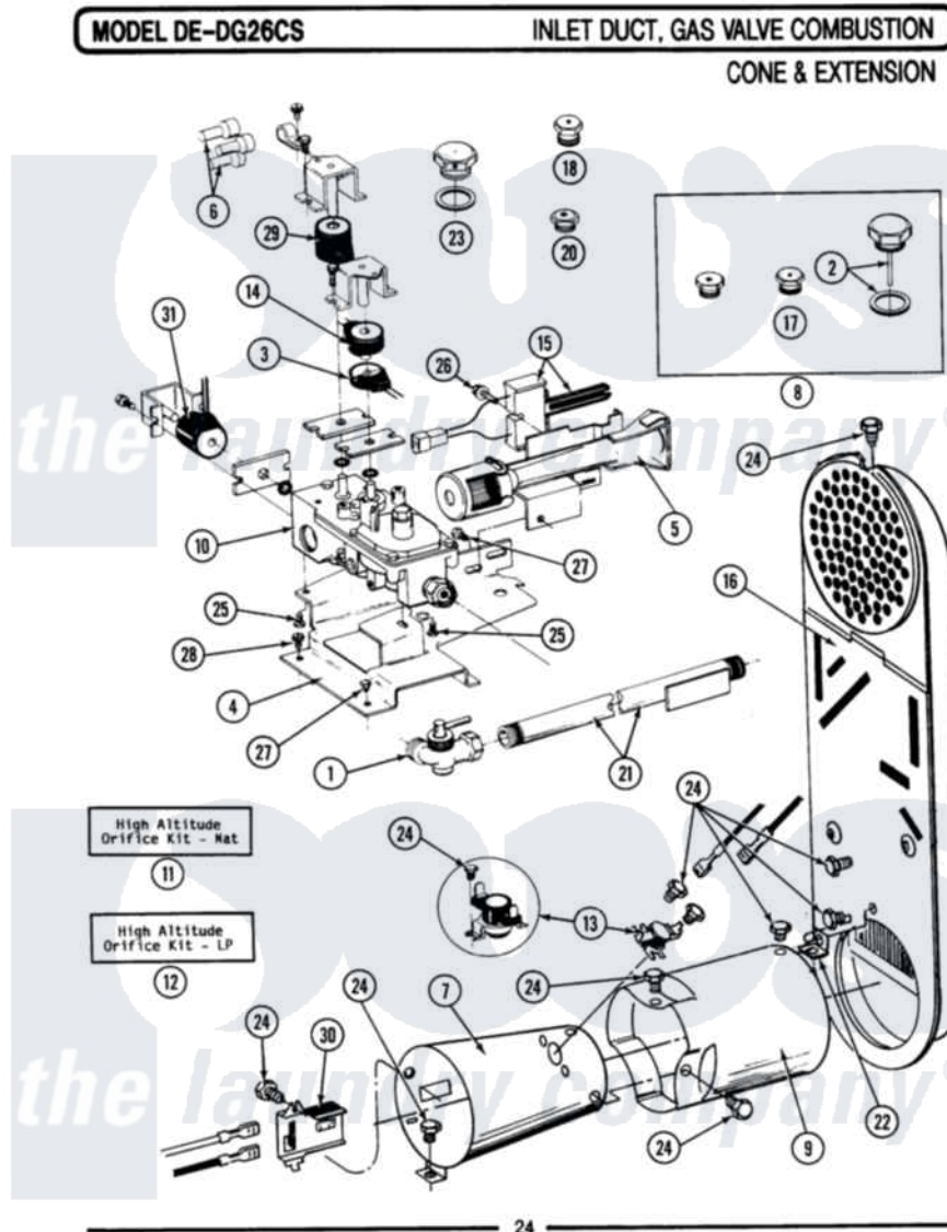
Maytag Commercial Maytag GDG26CS Dryer Parts Parts Diagram 10 - INLET DUCT, GAS VALVE, CONE & EXTENSION
