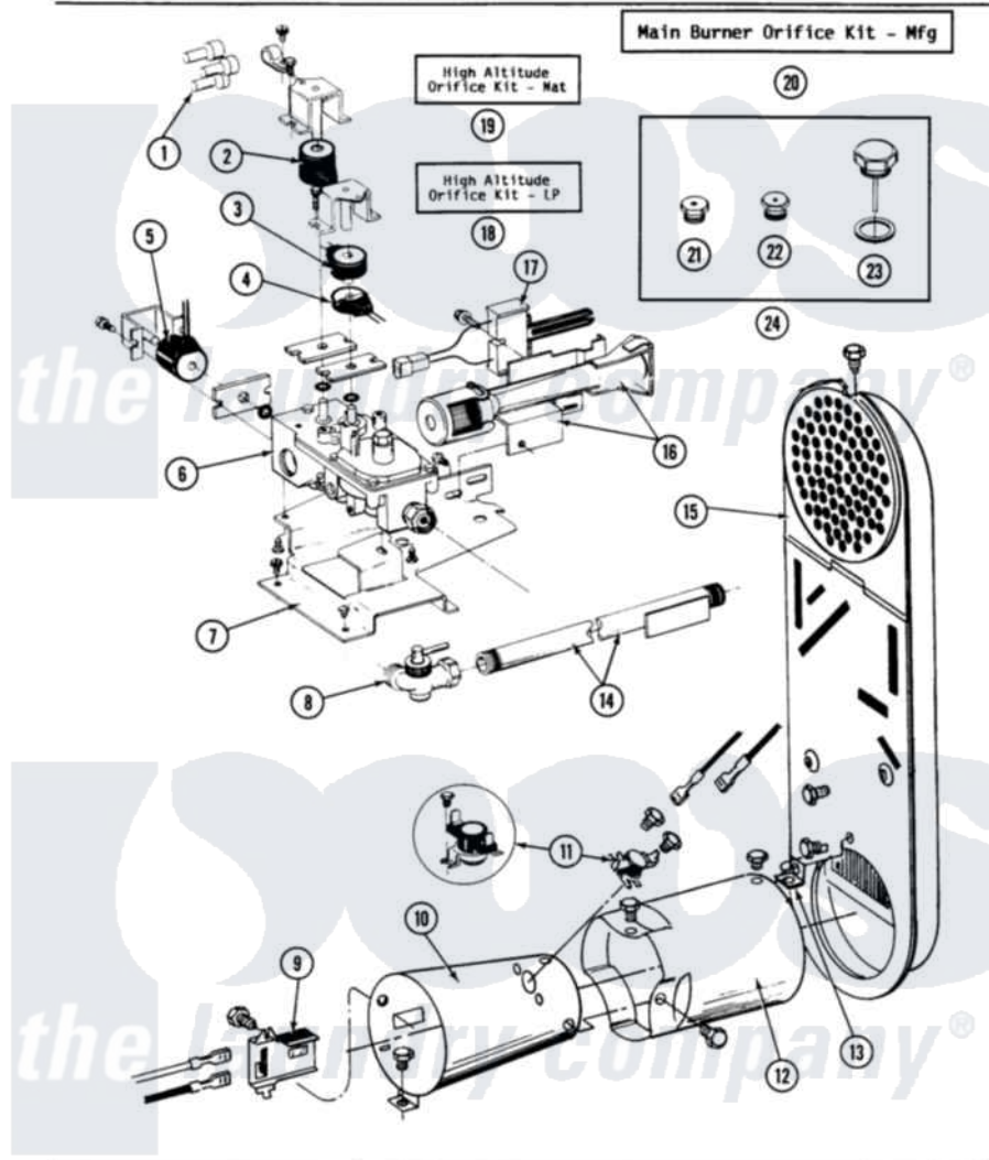
Maytag Commercial Maytag GDG27CT Dryer Parts Parts Diagram 11 - INLET DUCT, GAS VALVE & COMBUSTION CONE
