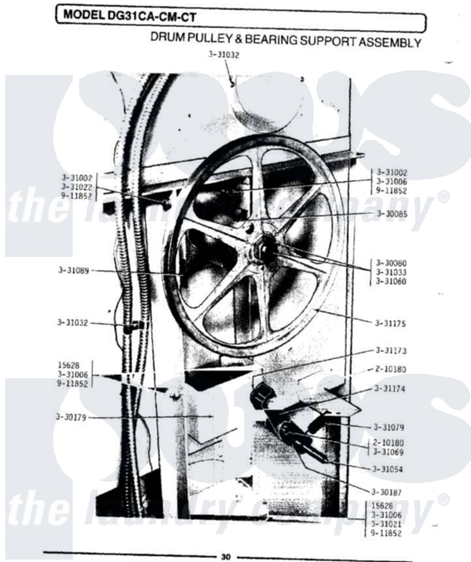
Maytag Commercial Maytag GDG31CA Dryer Parts Parts Diagram 11 - DRUM PULLEY & BEARING SUPPORT ASSEMBLY
