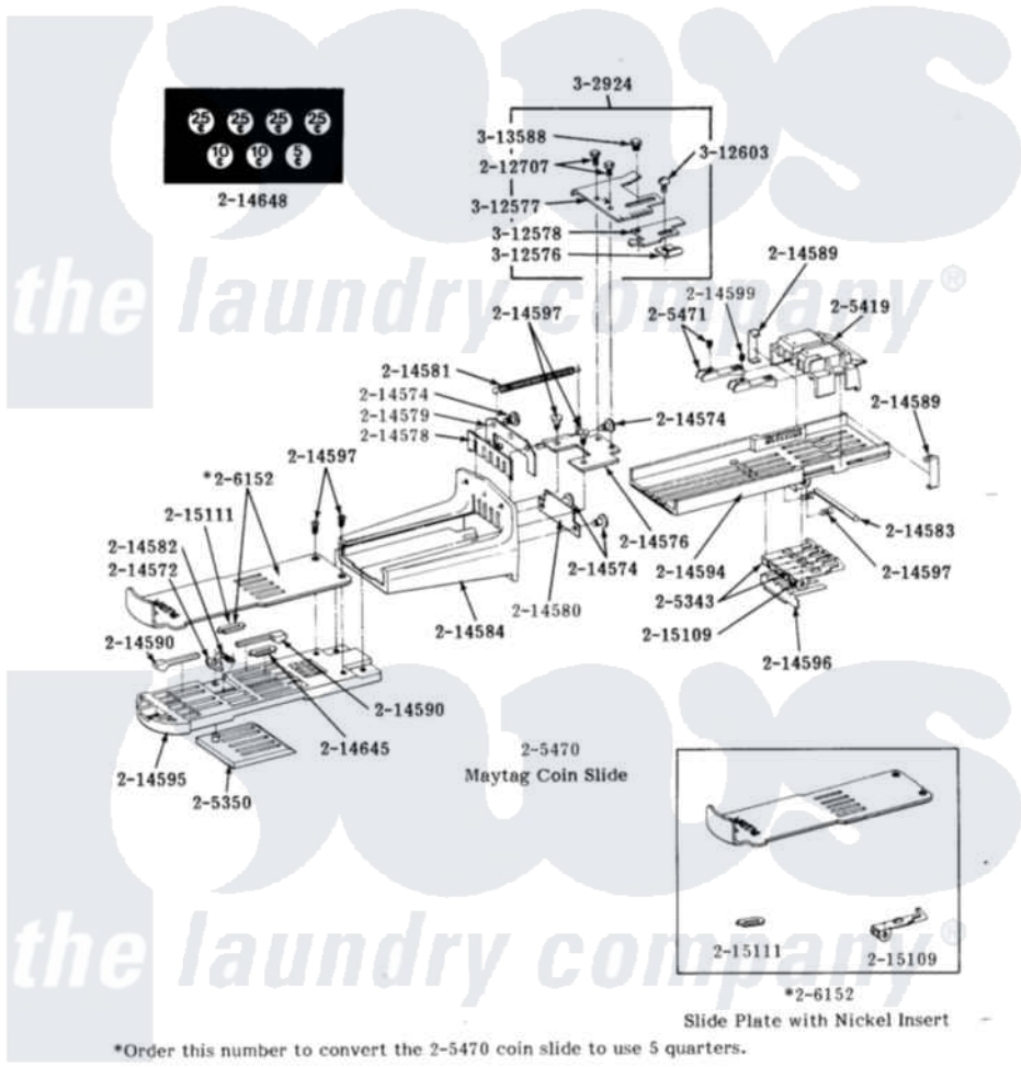
Maytag Commercial Maytag LDG21CS Dryer Parts Parts Diagram 05 - MAYTAG COIN SLIDE Click on the part number to view part
