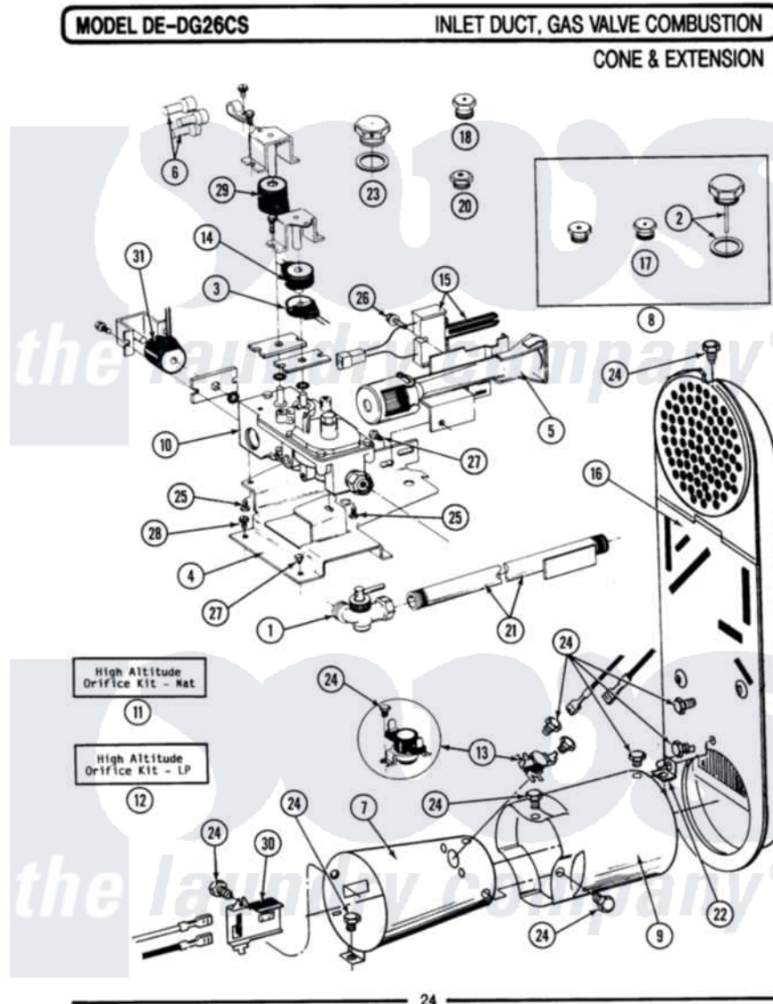
Maytag Commercial Maytag LDG26CS Dryer Parts Parts Diagram 10 - INLET DUCT, GAS VALVE, CONE & EXTENSION
