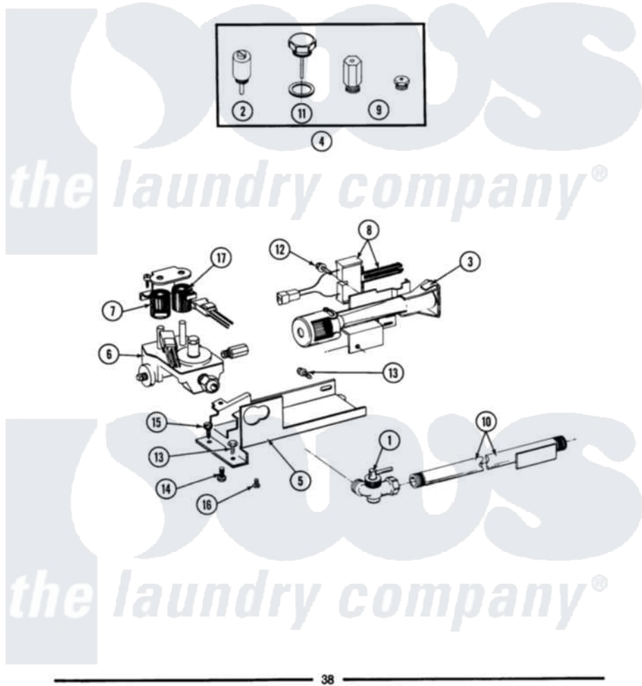
Maytag Commercial Maytag LDG26CS Dryer Parts Parts Diagram 11 - 50HZ GAS VALVE Click on the part number to view part
