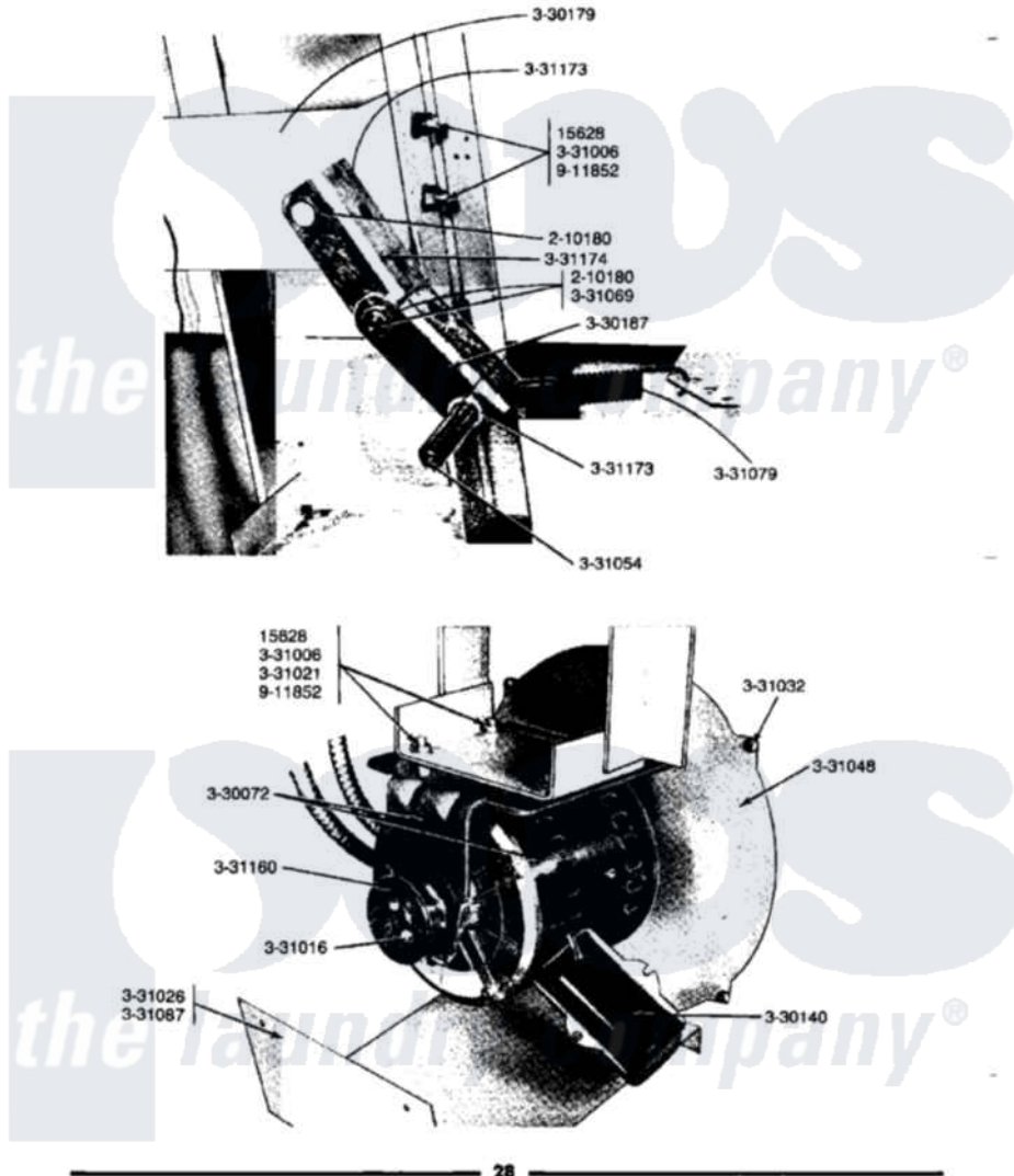
Maytag Commercial Maytag LDG33CM Dryer Parts Parts Diagram 12 - MOTOR & IDLER ARM ASSEMBLY Click on the part number to view part
