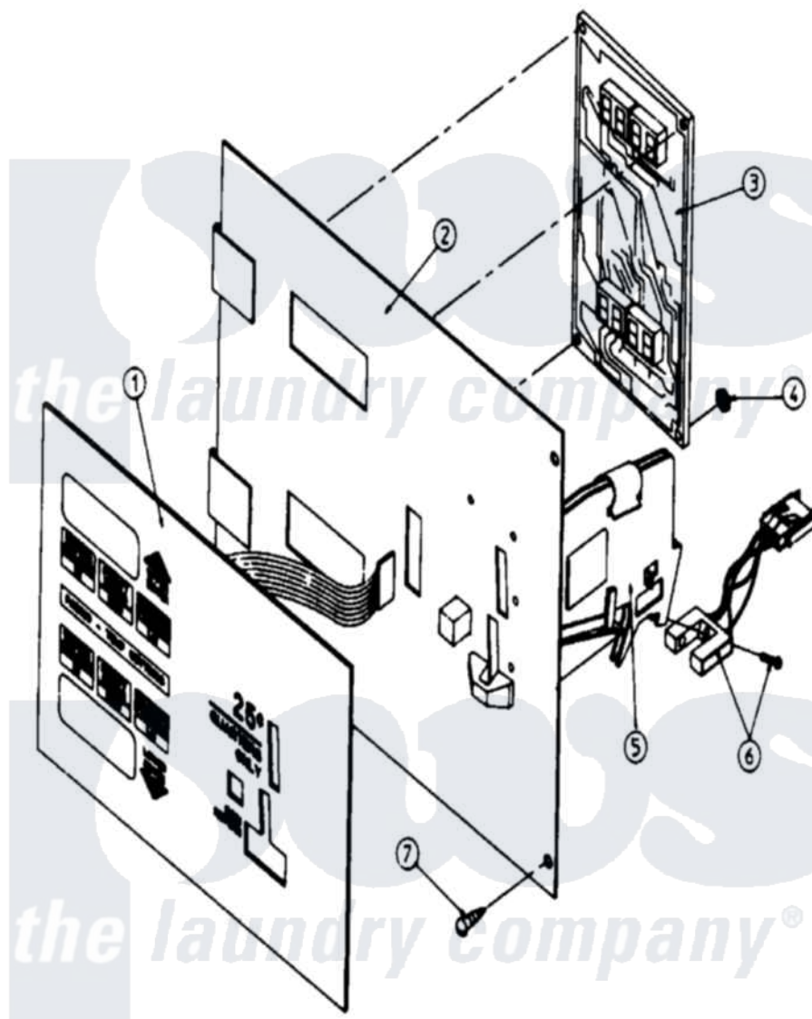
Maytag Commercial Maytag LDGS30PC1 Dryer Parts Parts Diagram 03 - CONTROL PANEL ASSEMBLY (DMC) Click on the part number to view part
