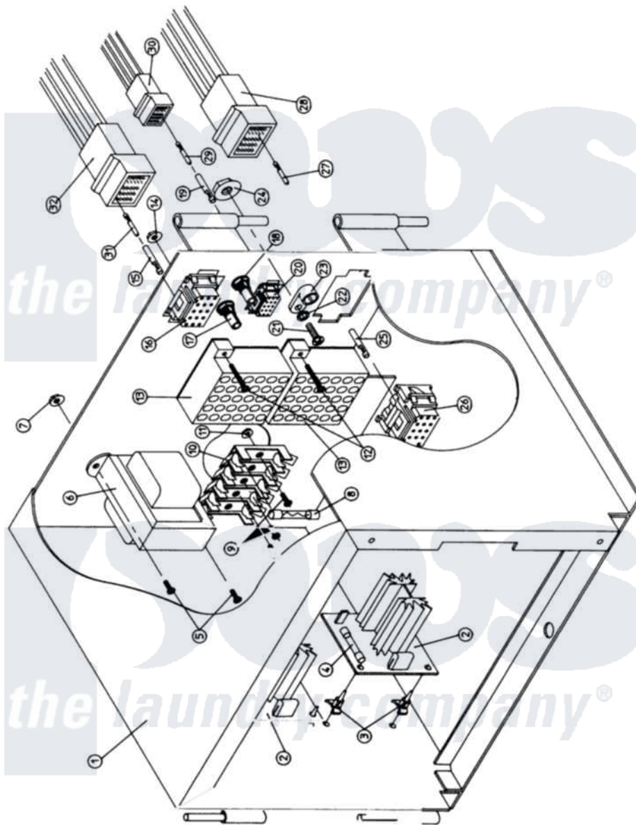
Maytag Commercial Maytag LDGS30PC1 Dryer Parts Parts Diagram 04 - DUAL CTRL MICROPROCESSOR (DMC) CNTRL BOX
