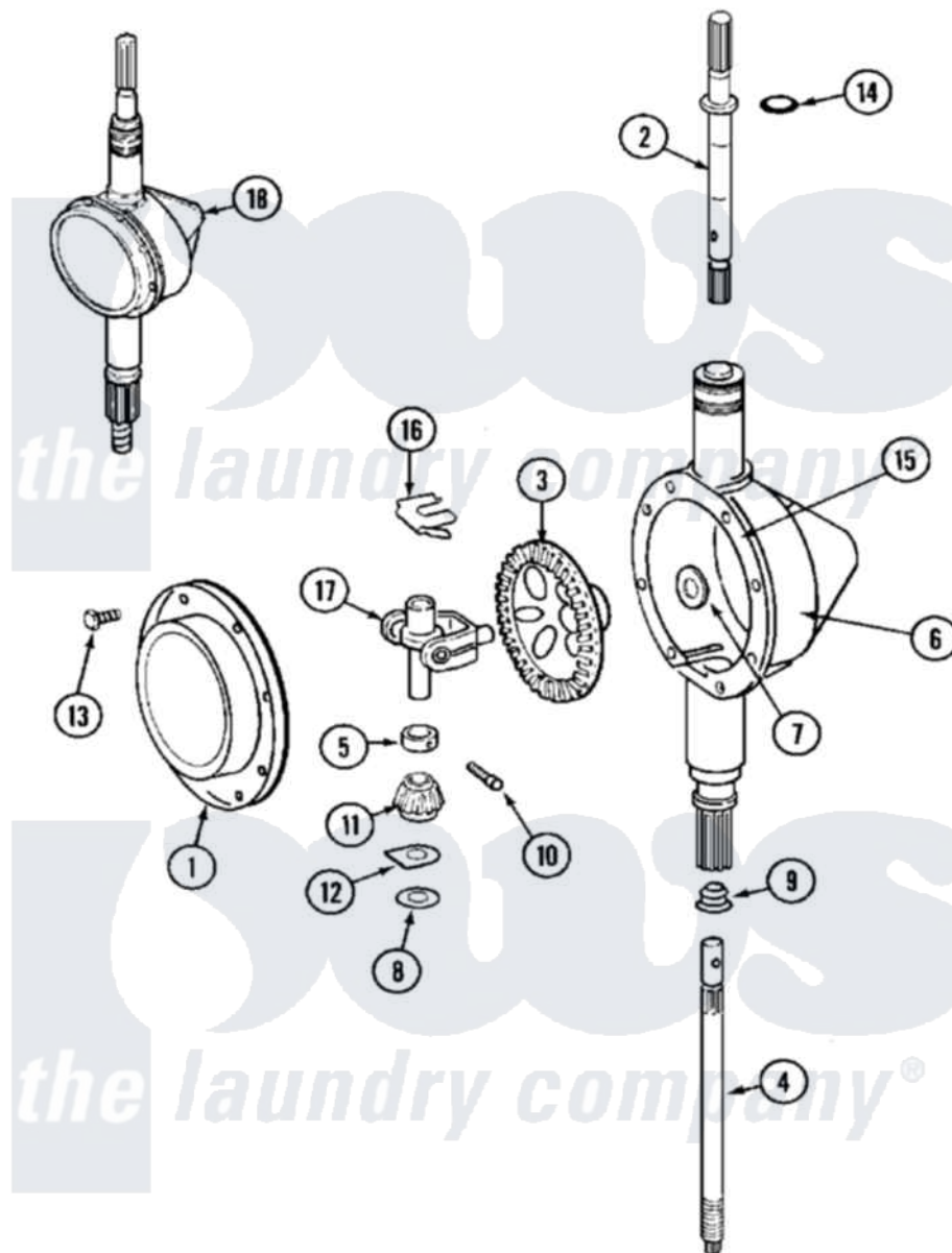
Maytag Commercial Maytag MAT10CSAGL Washer Parts Parts Diagram 07 - TRANSMISSION Click on the part number to view part
