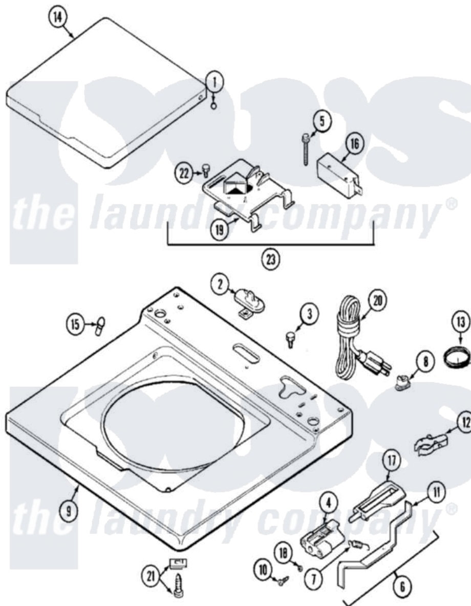
Maytag Commercial Maytag MAT10DAABW Washer Parts Parts Diagram 03 - TOP Click on the part number to view part
