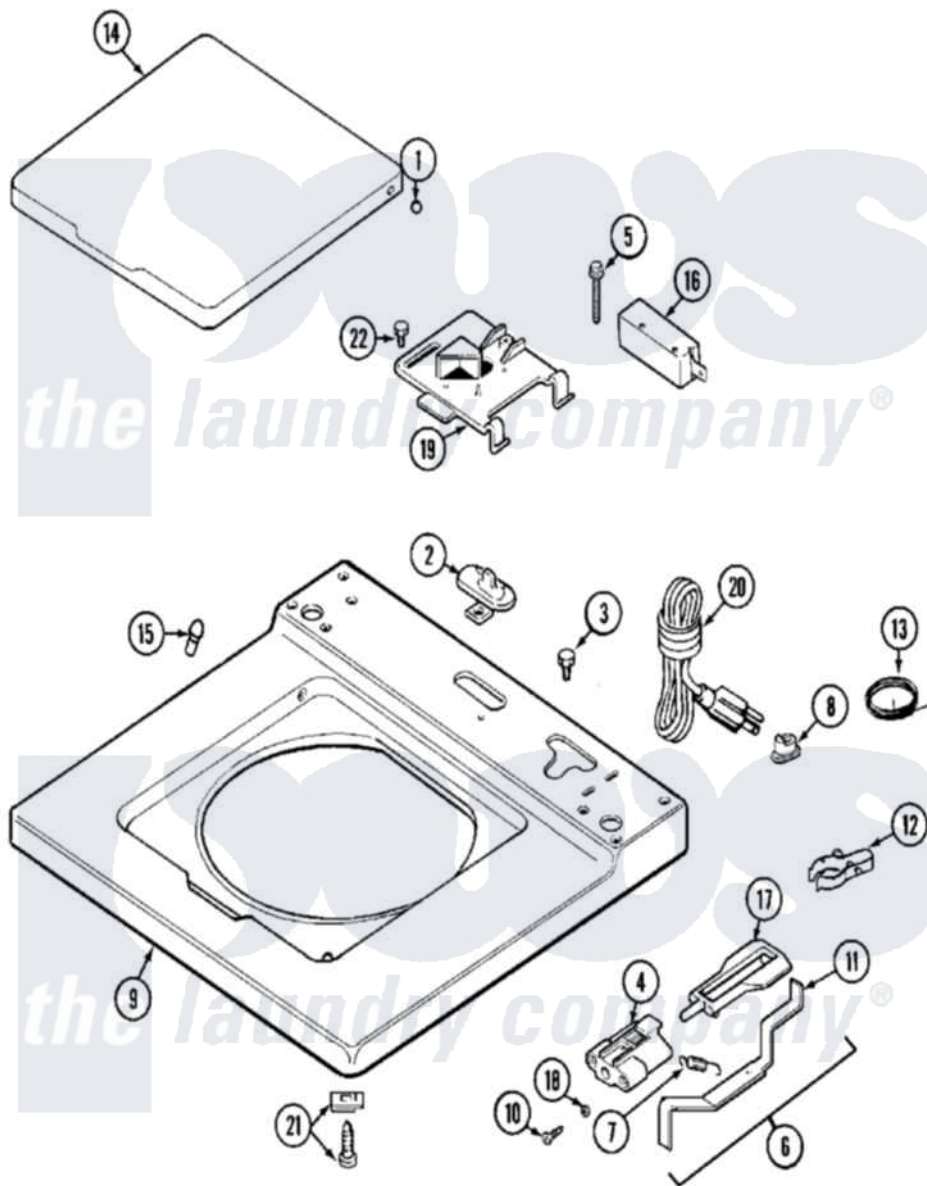
Maytag Commercial Maytag MAT10PDABL Washer Parts Parts Diagram 03 - TOP ASSEMBLY Click on the part number to view part
