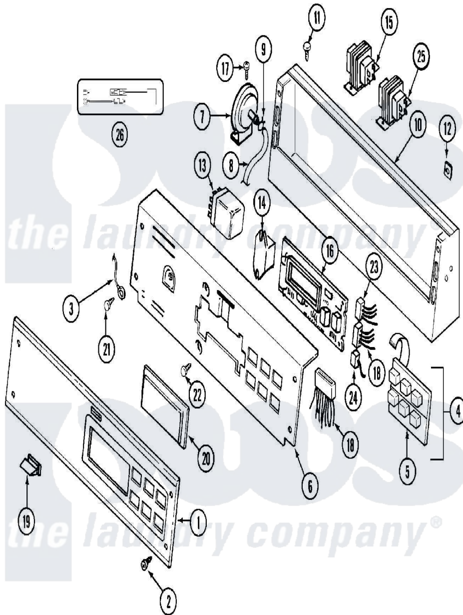
Maytag Commercial Maytag MAT10PSAAL Washer Parts Parts Diagram 01 - CONTROL PANEL Click on the part number to view part
