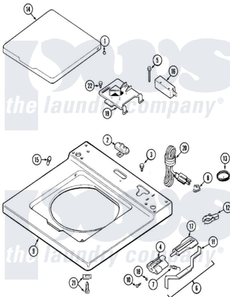
Maytag Commercial Maytag MAT10PSAAL Washer Parts Parts Diagram 02 - TOP Click on the part number to view part
