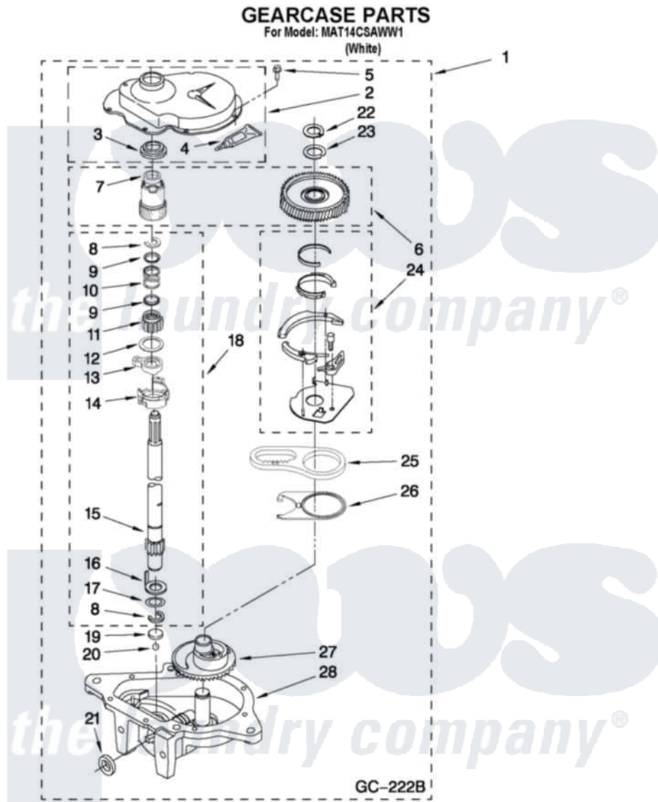
Maytag Commercial Maytag MAT14CSAWW1 Washer Parts Parts Diagram 09 - GEARCASE PARTS Click on the part number to view part
