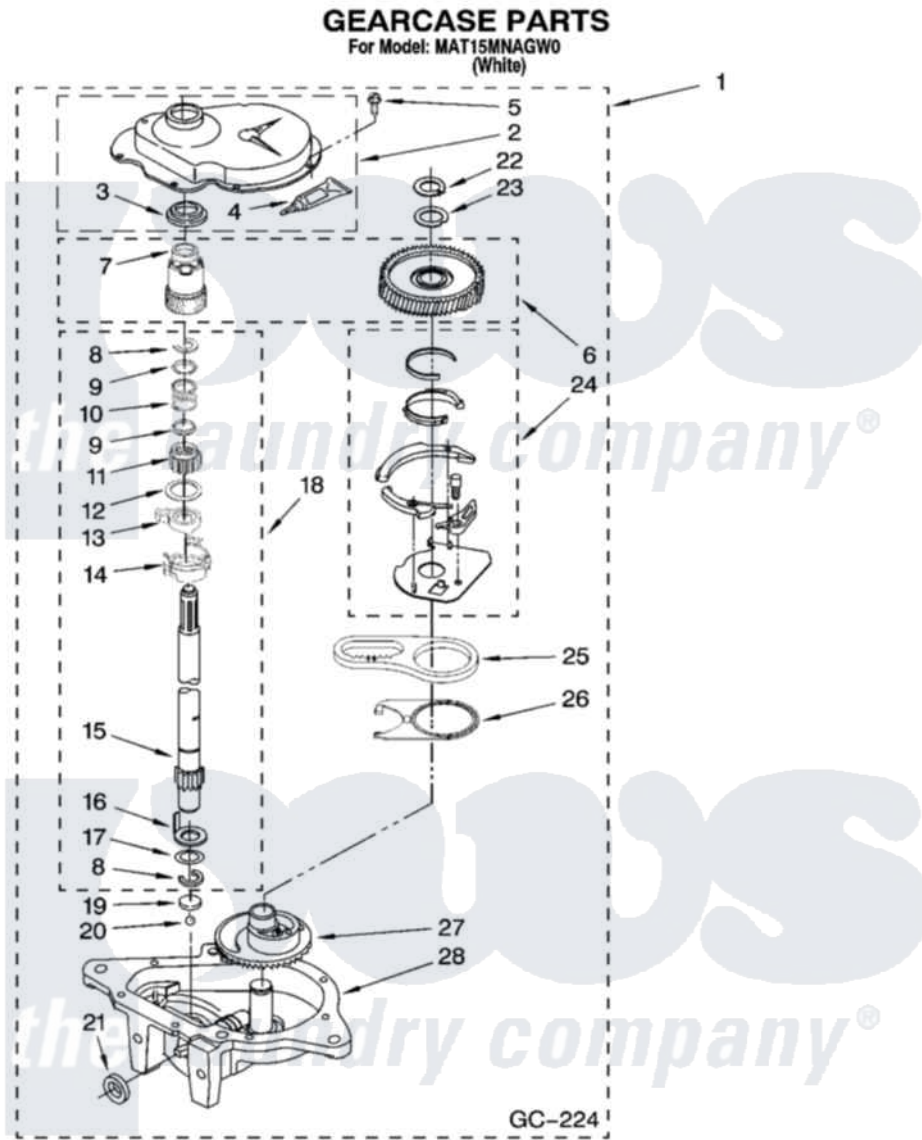
Maytag Commercial Maytag MAT15MNAGW0 Washer Parts Parts Diagram 09 - GEARCASE PARTS Click on the part number to view part
