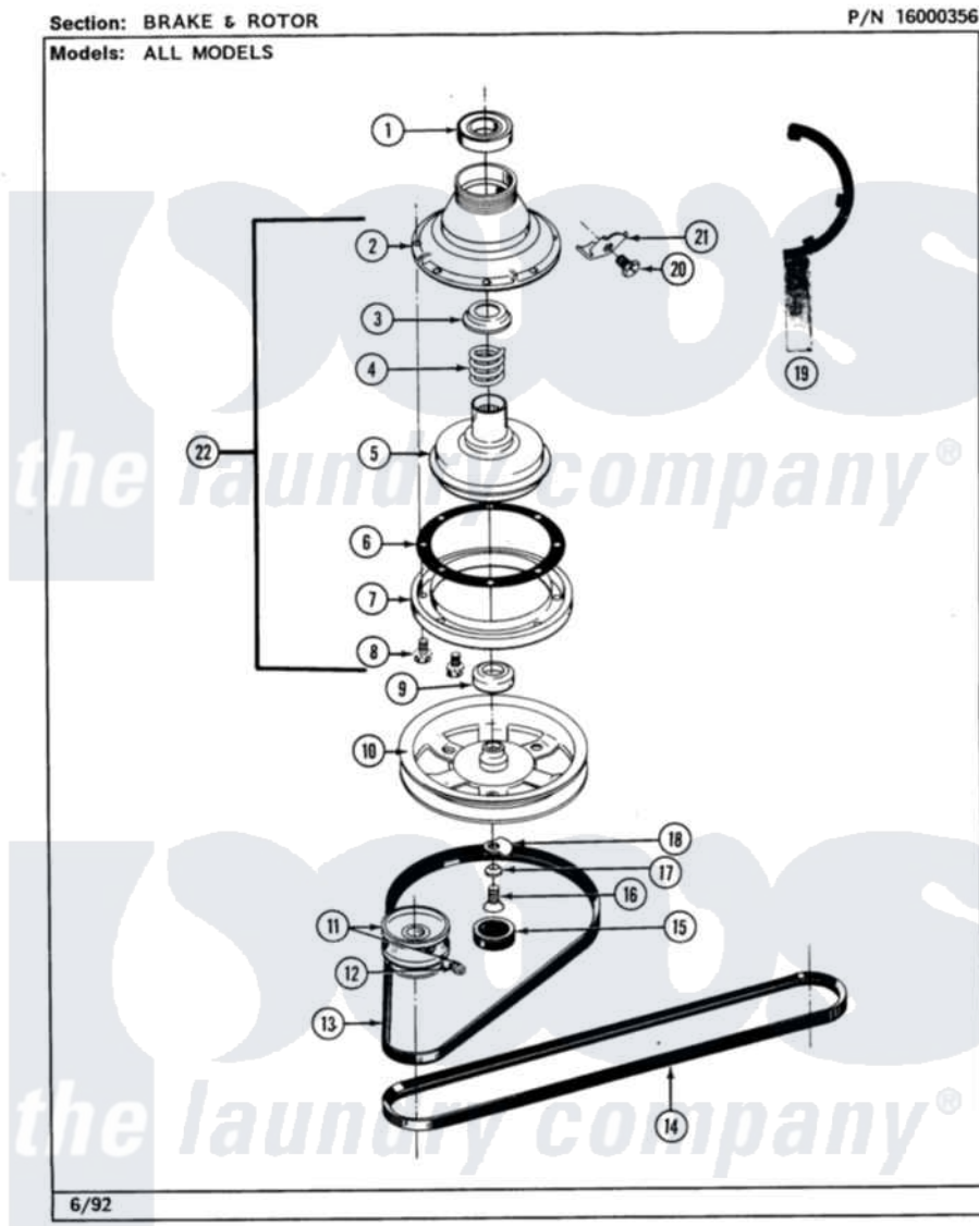
Maytag Commercial Maytag MAT23PCAAW Washer Parts Parts Diagram 09 - BRAKE & ROTOR Click on the part number to view part
