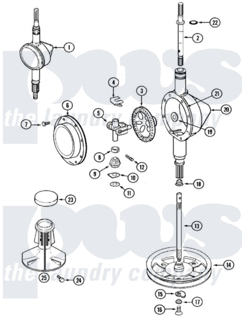
Maytag Commercial Maytag MAT25CTAAW Washer Parts Parts Diagram 08 - TRANSMISSION Click on the part number to view part
