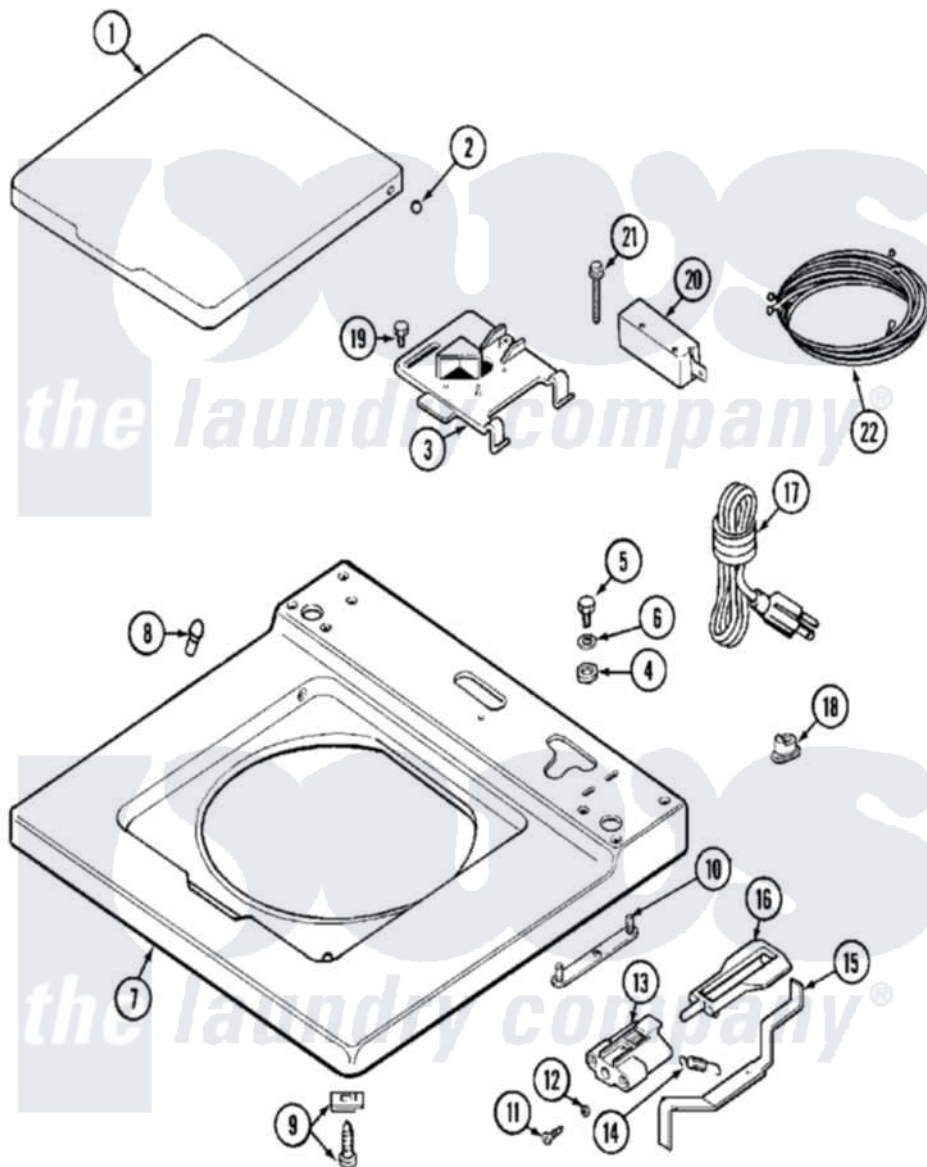
Maytag Commercial Maytag MAT26MNAAW Washer Parts Parts Diagram 02 - TOP Click on the part number to view part
