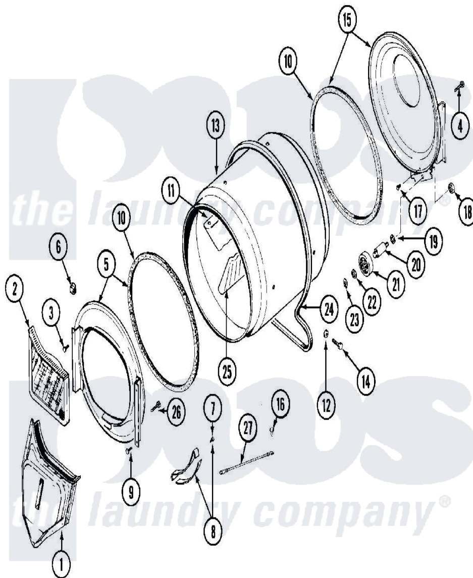
Maytag Commercial Maytag MDE10PSAGL Dryer Parts Parts Diagram 06 - TUMBLER Click on the part number to view part
