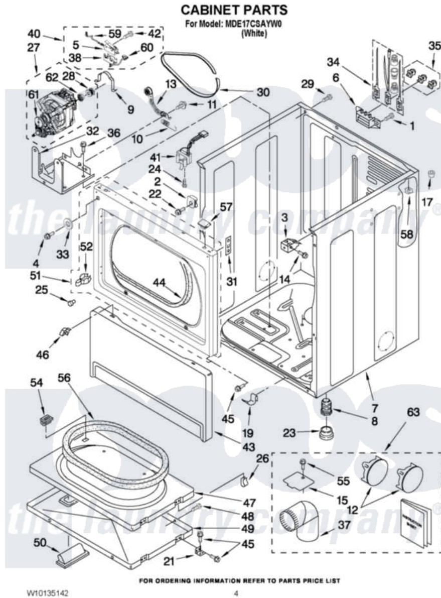
Maytag Commercial Maytag MDE17CSAYW0 Dryer Parts Parts Diagram 02 - CABINET PARTS Click on the part number to view part
