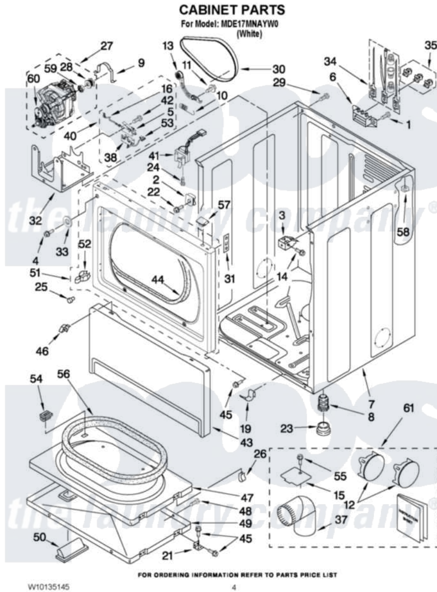
Maytag Commercial Maytag MDE17MNAYW0 Dryer Parts Parts Diagram 02 - CABINET PARTS Click on the part number to view part
