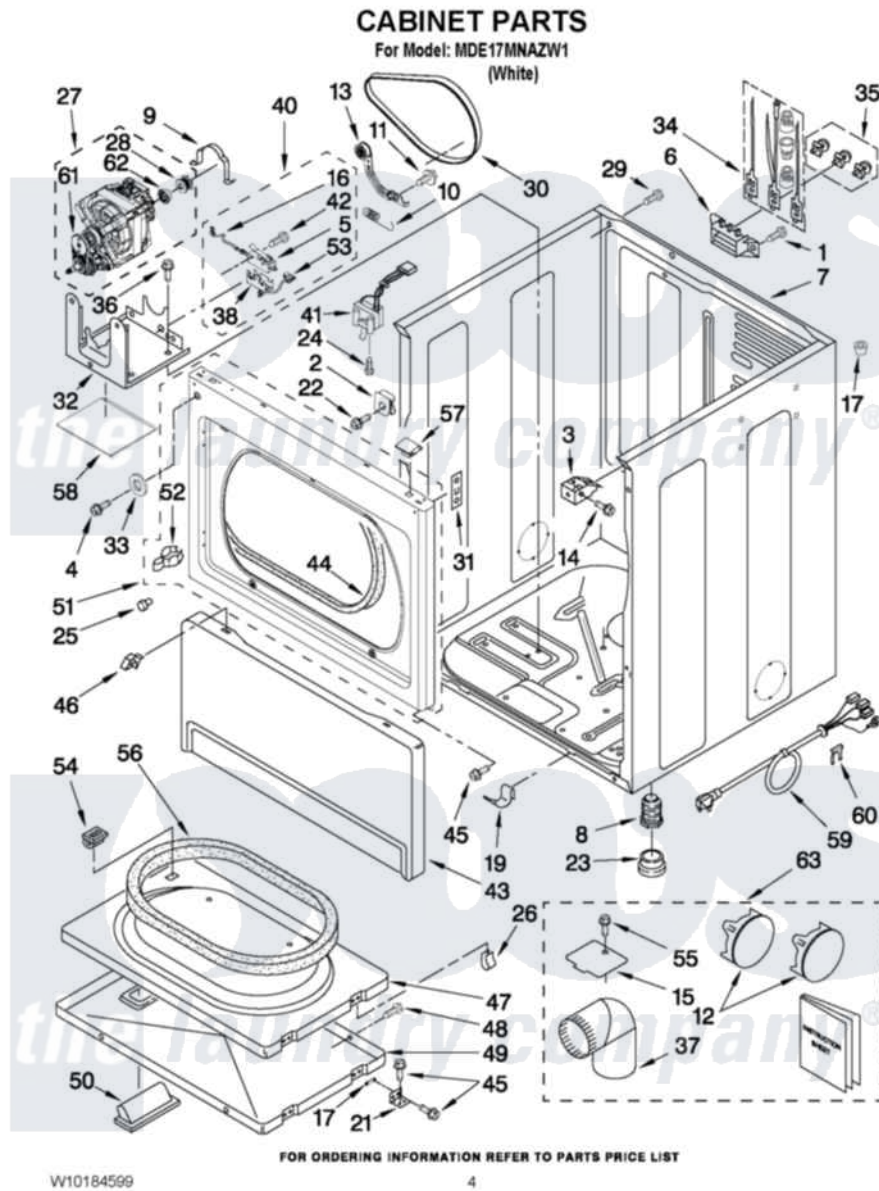
Maytag Commercial Maytag MDE17MNAZW1 Dryer Parts Parts Diagram 02 - CABINET PARTS Click on the part number to view part
