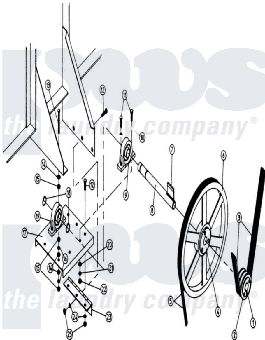
Maytag Commercial Maytag MDG100PN1L Dryer Parts Parts Diagram 10 - IDLER BEARING MOUNT ASSEMBLY Click on the part number to view part
