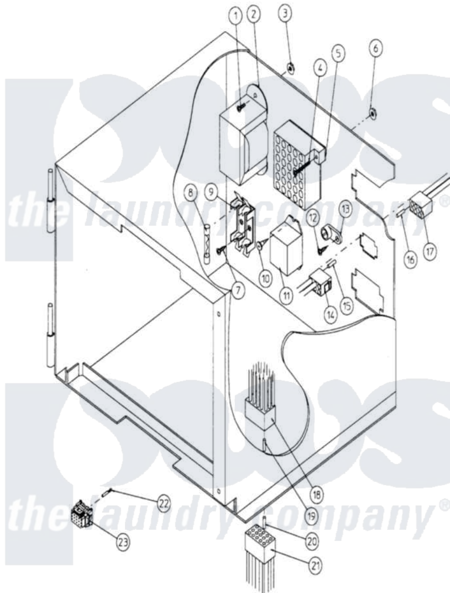
Maytag Commercial Maytag MDG120P1HW Dryer Parts Parts Diagram 02 - MICROPROCESSOR CONTROL BOX ASSY
