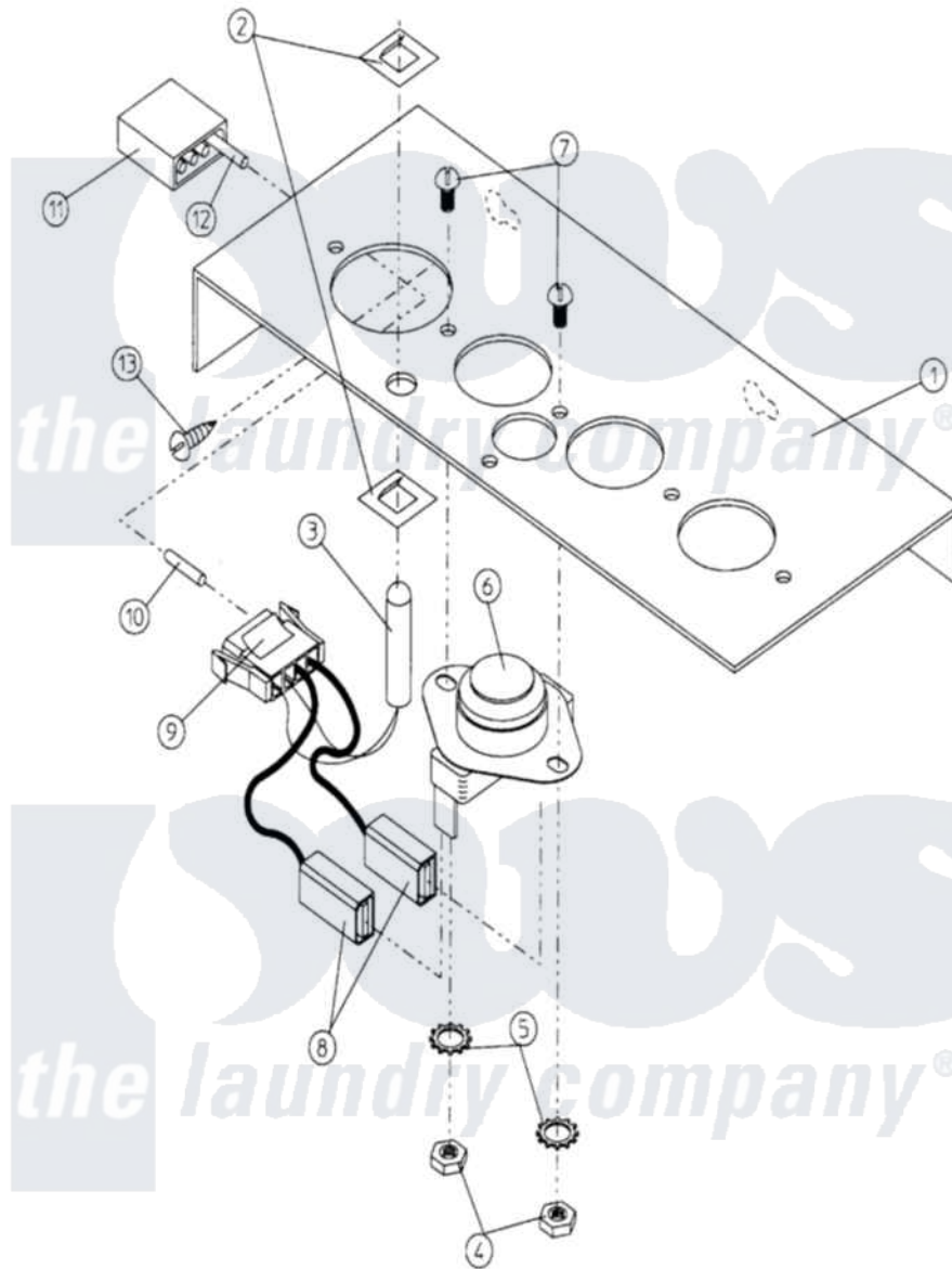
Maytag Commercial Maytag MDG120P1HW Dryer Parts Parts Diagram 07 - MICROPROCESSOR TEMP SENSOR BRKT ASSY
