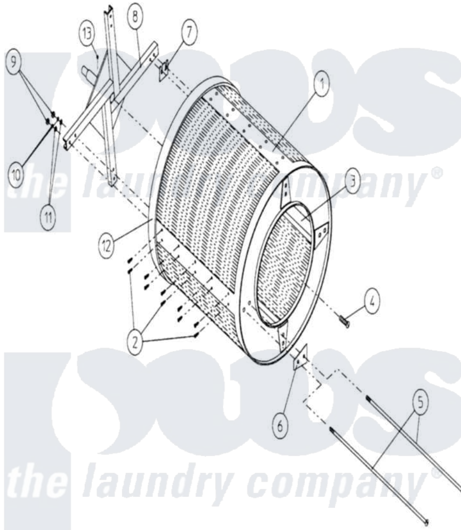
Maytag Commercial Maytag MDG120P1HW Dryer Parts Parts Diagram 08 - BASKET (TUMBLER) SUPPORT ASSEMBLIES
