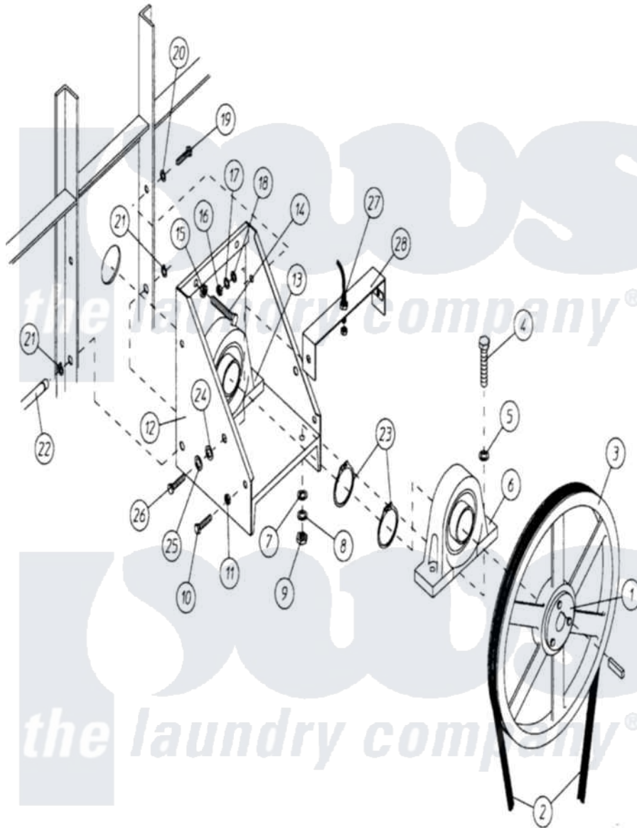
Maytag Commercial Maytag MDG120P1HW Dryer Parts Parts Diagram 09 - TUMBLER BEARING MOUNT ASSEMBLY Click on the part number to view part
