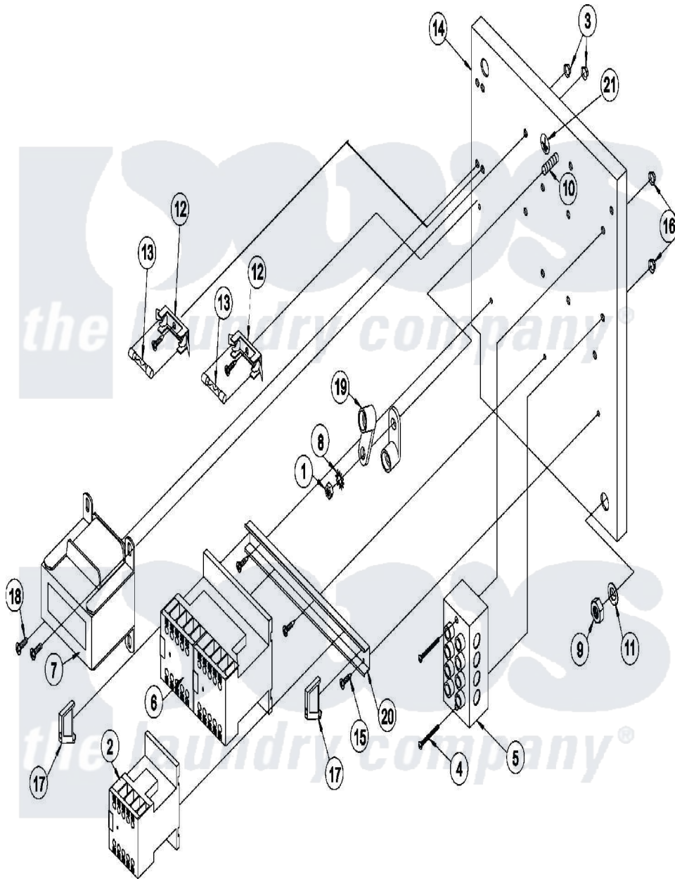
Maytag Commercial Maytag MDG120PHVW Dryer Parts Parts Diagram 15 - REVERSING PANEL (208-240V) Click on the part number to view part
