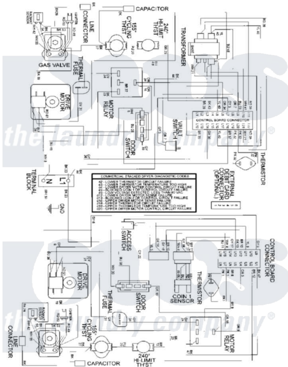
Maytag Commercial Maytag MDG13PDBBL Dryer Parts Parts Diagram 08 - WIRING INFORMATION Click on the part number to view part
