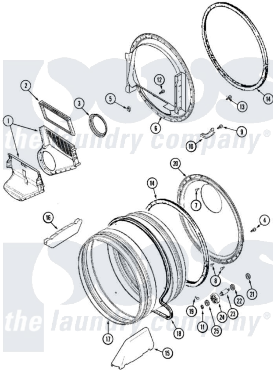
Maytag Commercial Maytag MDG16PDAXA Dryer Parts Parts Diagram 07 - TUMBLER Click on the part number to view part
