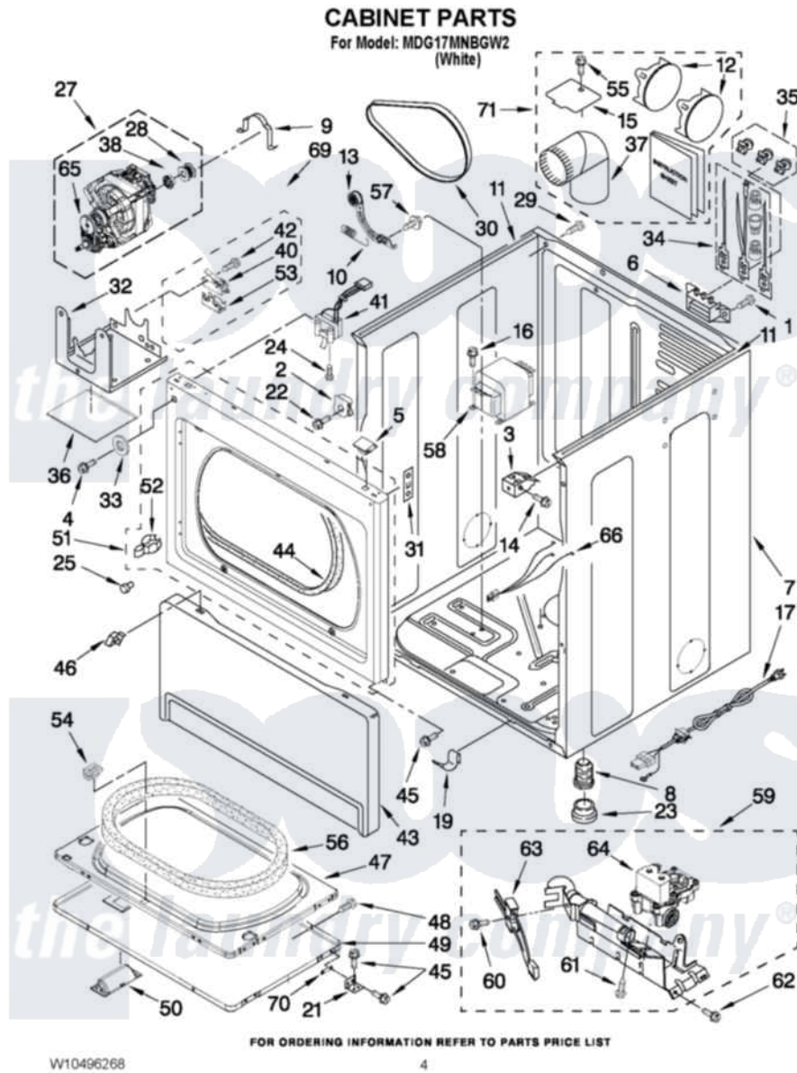
Maytag Commercial Maytag MDG17MNBGW2 Dryer Parts Parts Diagram 02 - CABINET PARTS Click on the part number to view part
