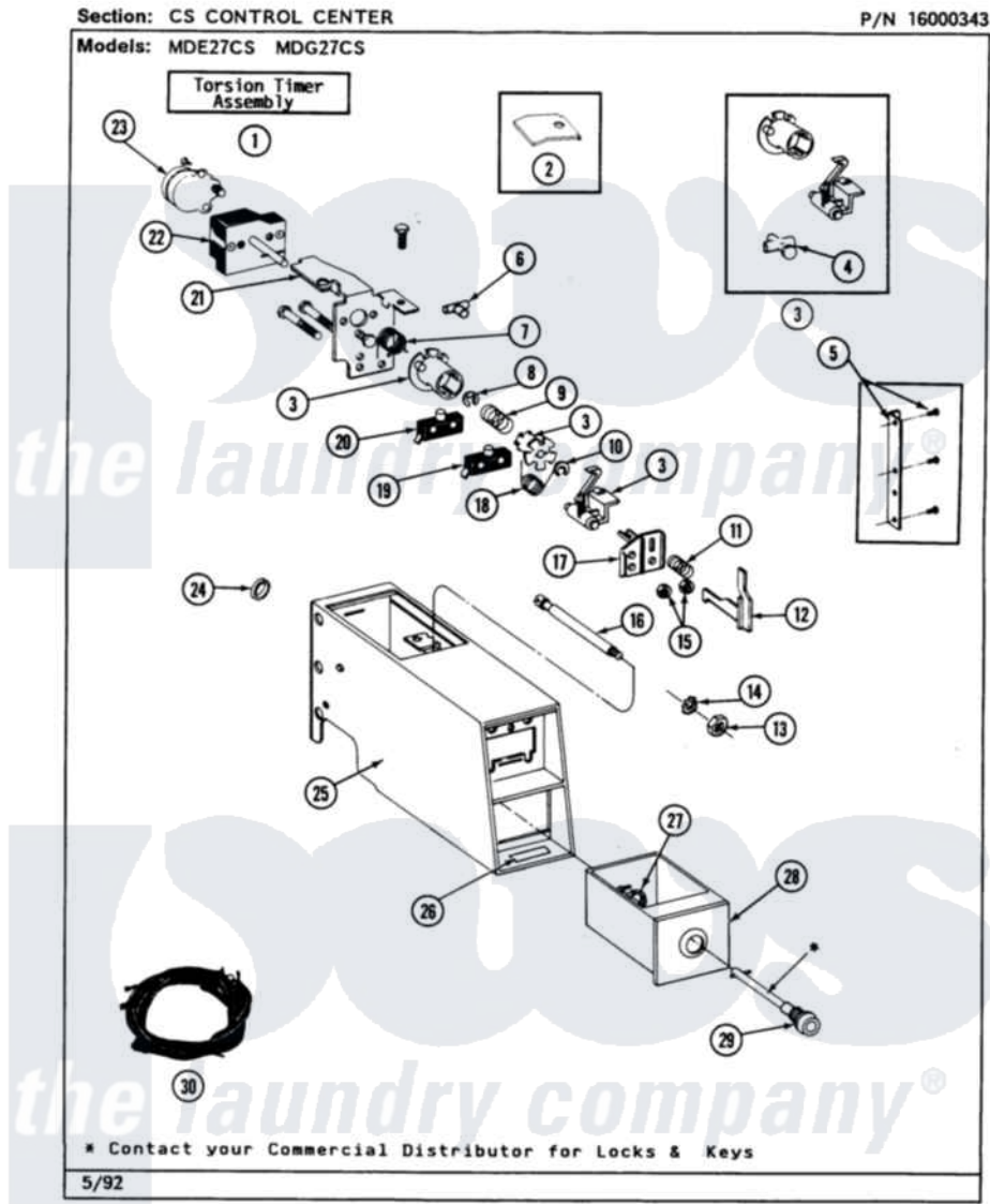
Maytag Commercial Maytag MDG27CSAGL Dryer Parts Parts Diagram 04 - CONTROL CENTER Click on the part number to view part
