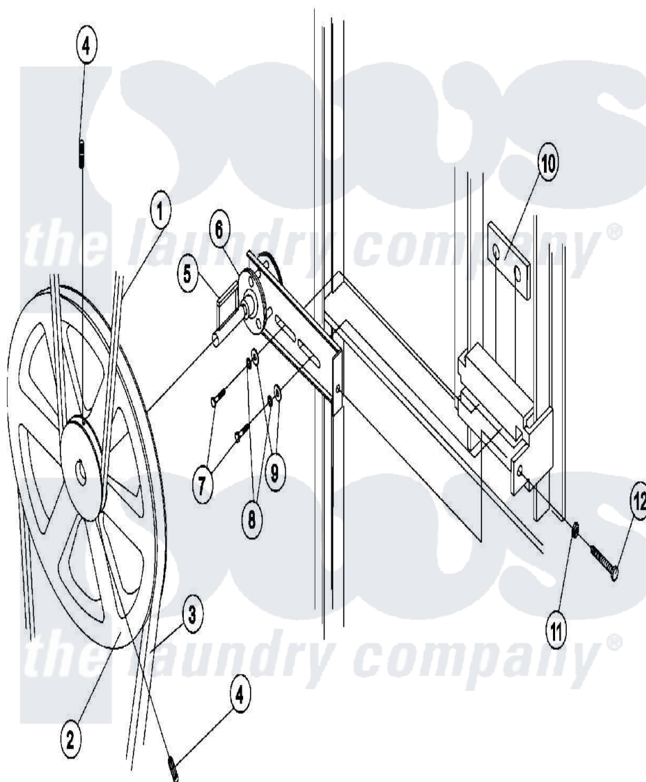
Maytag Commercial Maytag MDG30MNVWW Dryer Parts Parts Diagram 12 - IDLER BEARING Click on the part number to view part
