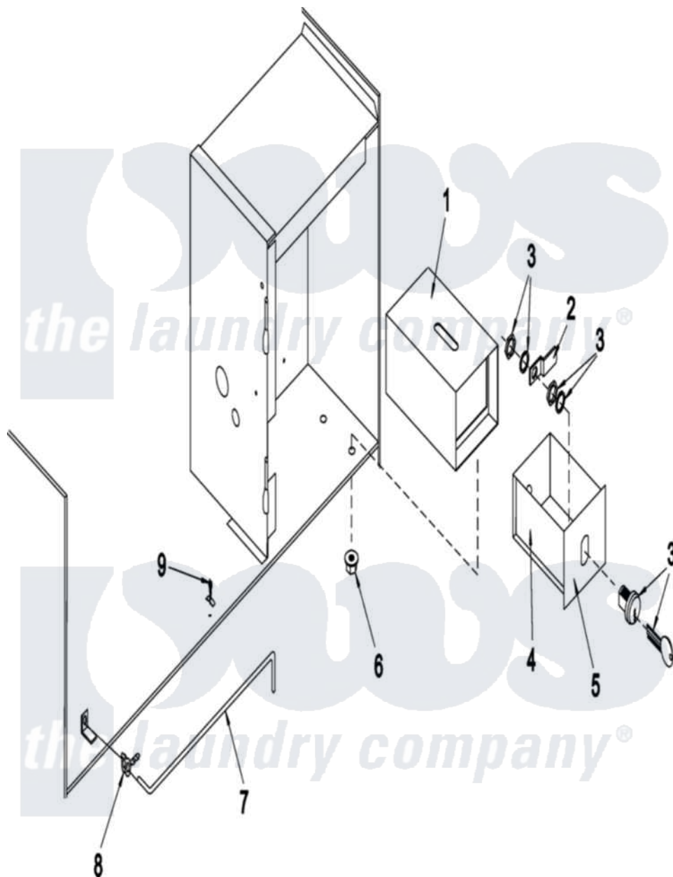
Maytag Commercial Maytag MDG30PCCWQ Dryer Parts Parts Diagram 03 - COIN VAULT Click on the part number to view part
