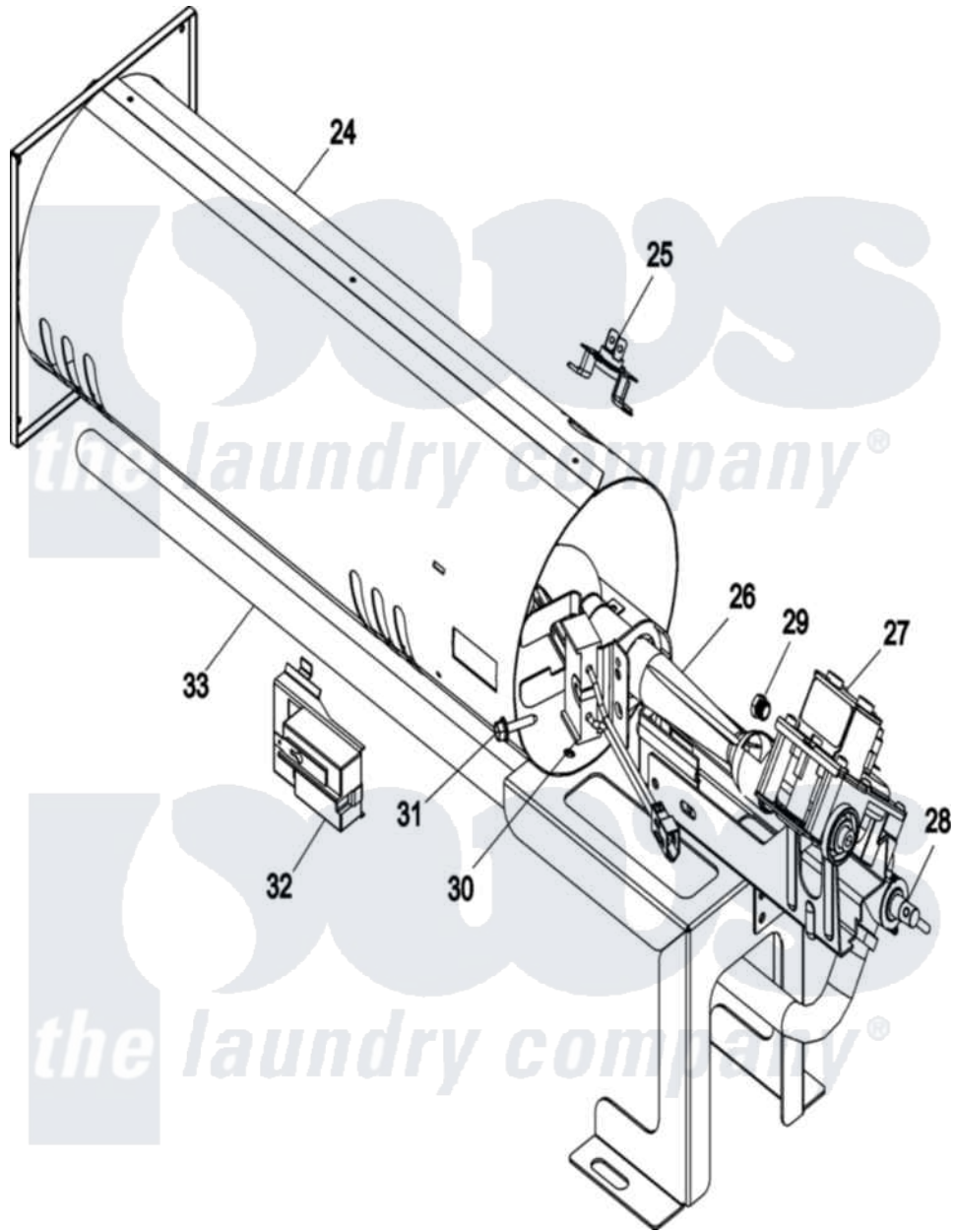
Maytag Commercial Maytag MDG31PDAWW Dryer Parts Parts Diagram 05 - BURNER Click on the part number to view part
