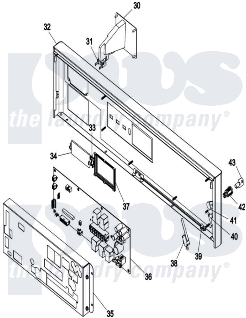
Maytag Commercial Maytag MDG31PDSWW Dryer Parts Parts Diagram 03 - PANEL, CONTROL Click on the part number to view part
