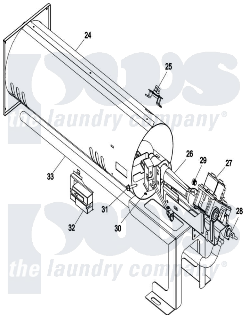
Maytag Commercial Maytag MDG31PNAWW Dryer Parts Parts Diagram 05 - BURNER Click on the part number to view part
