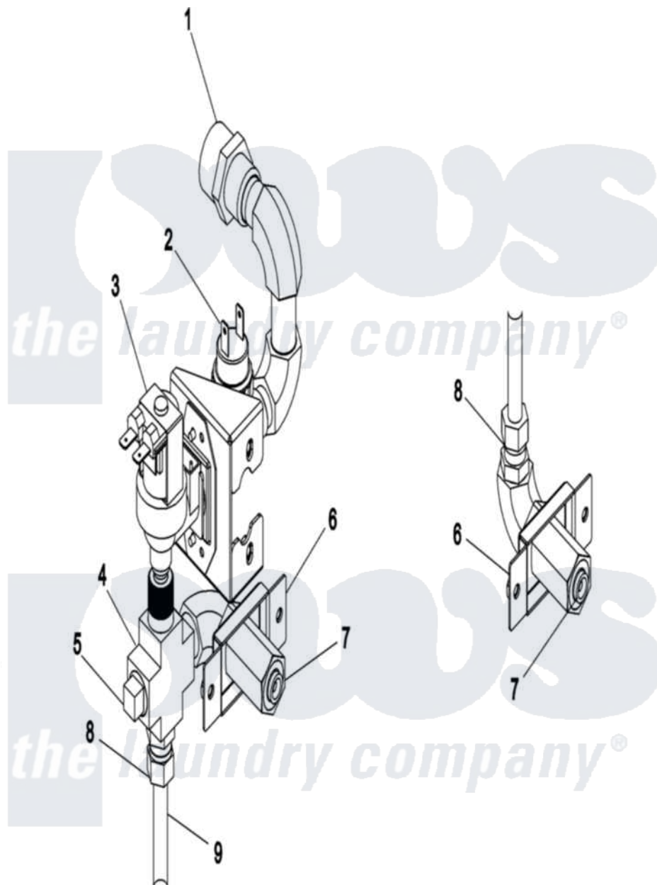
Maytag Commercial Maytag MDG31PNSWW Dryer Parts Parts Diagram 08 - SAFE SYSTEM ASSEMBLY Click on the part number to view part
