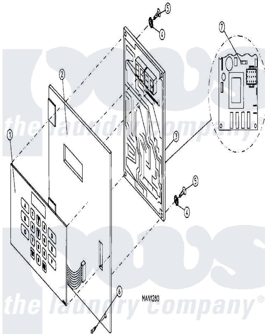
Maytag Commercial Maytag MDG50PN1AW Dryer Parts Parts Diagram 01 - CONTROL PANEL ASSEMBLY (PN1A/PN2V)
