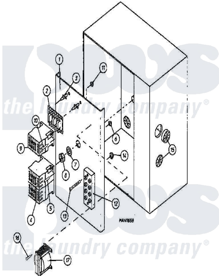
Maytag Commercial Maytag MDG50PN2VW Dryer Parts Parts Diagram 16 - REAR CONTROL BOX ASSEMBLY (PN2VW)
