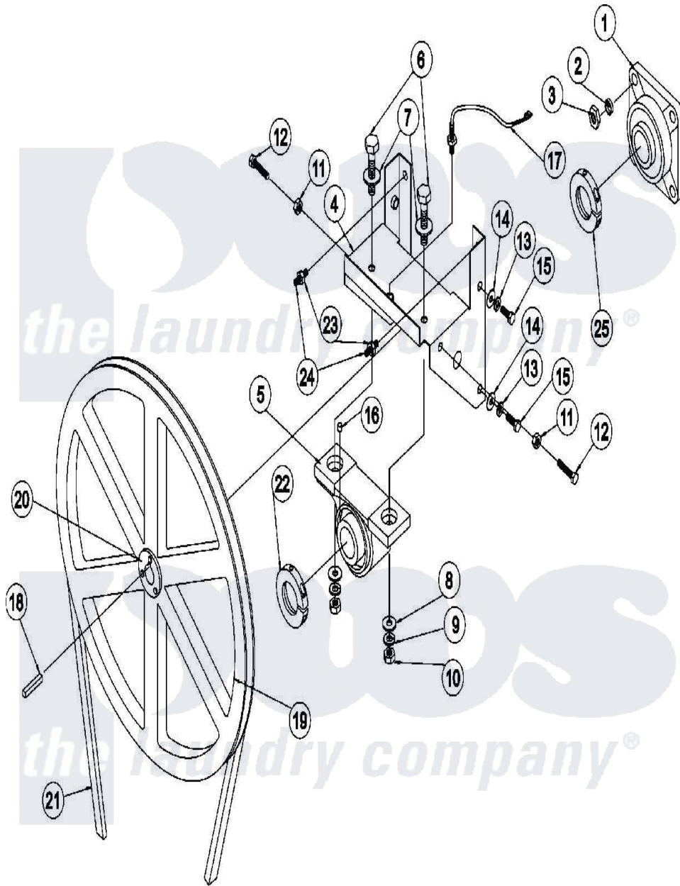
Maytag Commercial Maytag MDG50PNHWW Dryer Parts Parts Diagram 10 - TUMBLER BEARING Click on the part number to view part
