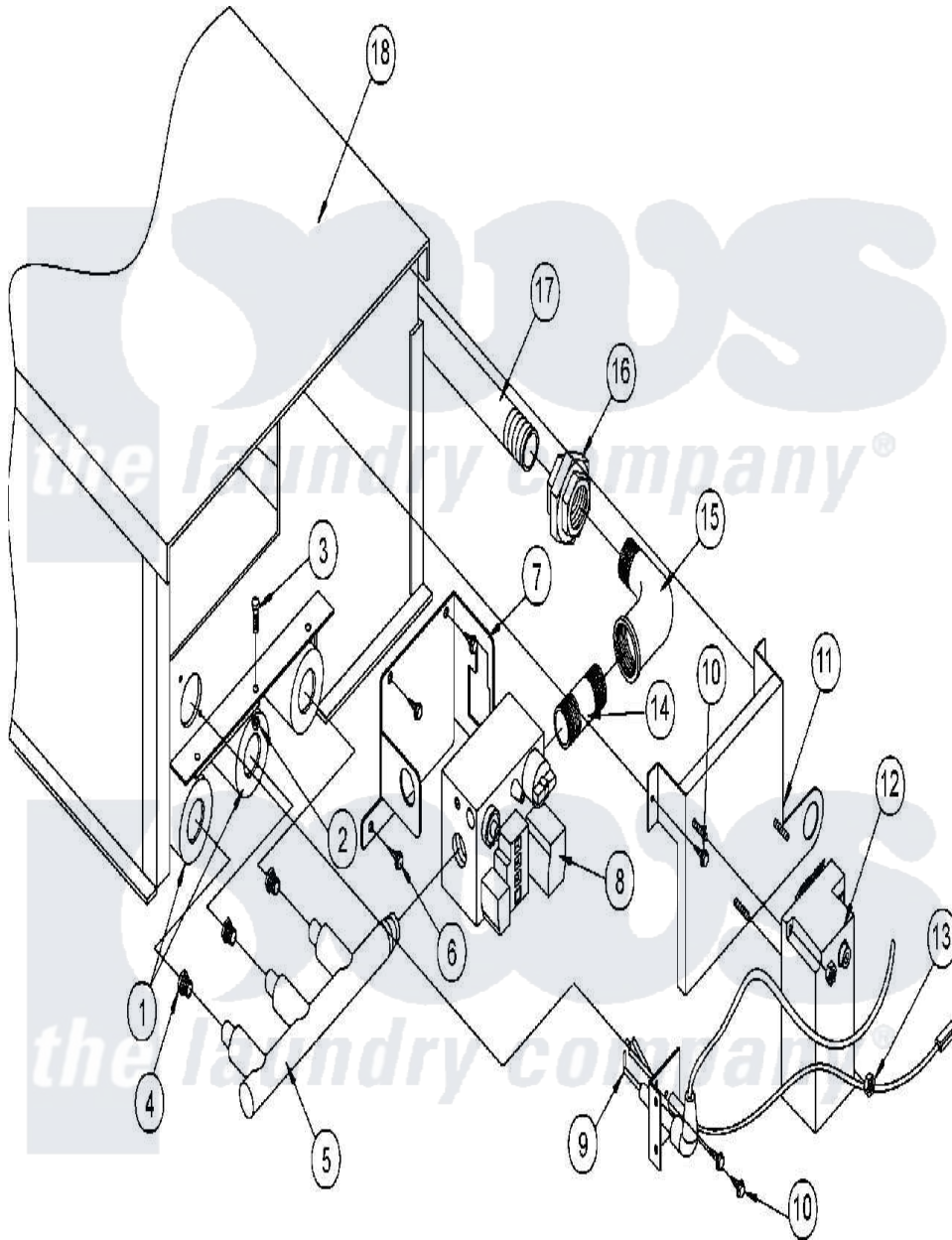
Maytag Commercial Maytag MDG50PNHWW Dryer Parts Parts Diagram 12 - GAS BURNER Click on the part number to view part
