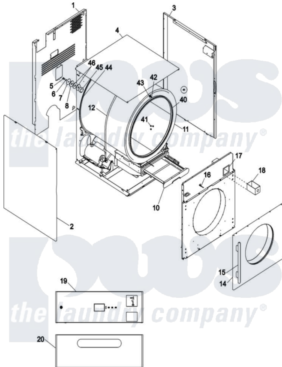
Maytag Commercial Maytag MDG51PNSWW Dryer Parts Parts Diagram 01 - CABINET
