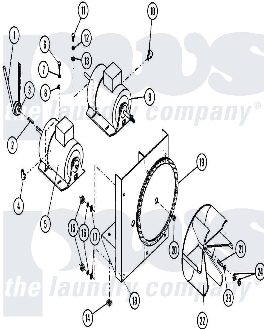
Maytag Commercial Maytag MDG75MNAWW Dryer Parts Parts Diagram 16 - MOTOR & MOUNT ASSEMBLY (PN2V) Click on the part number to view part
