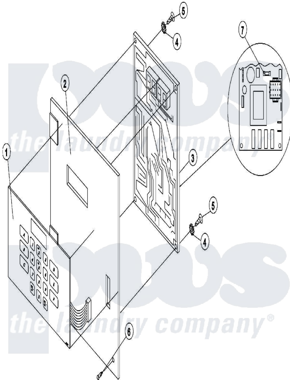
Maytag Commercial Maytag MDG75MNVWW Dryer Parts Parts Diagram 02 - CONTROL PANEL (MICROPROCESSOR) Click on the part number to view part
