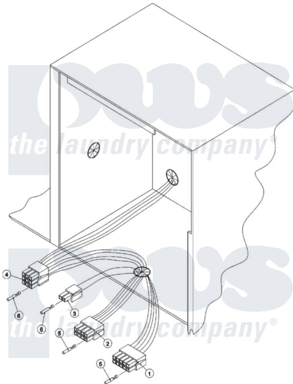
Maytag Commercial Maytag MDG76PCBWW Dryer Parts Parts Diagram 03 - CONTROL BOX ASSY Click on the part number to view part
