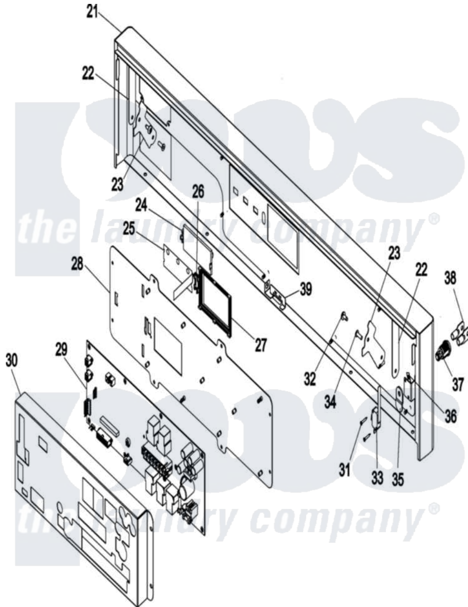
Maytag Commercial Maytag MDG77PNAWW Dryer Parts Parts Diagram 02 - CONTROL PANEL Click on the part number to view part
