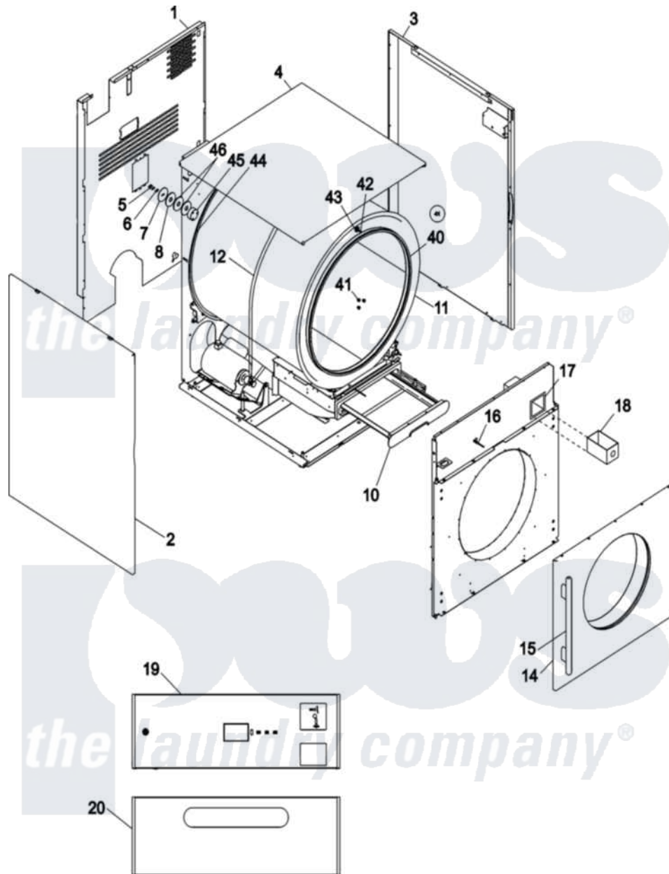
Maytag Commercial Maytag MDG77PNSWW Dryer Parts Parts Diagram 01 - CABINET Click on the part number to view part
